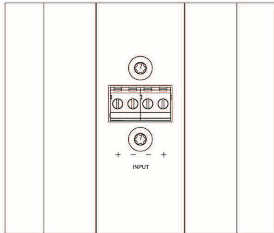
Phoenix connector input
